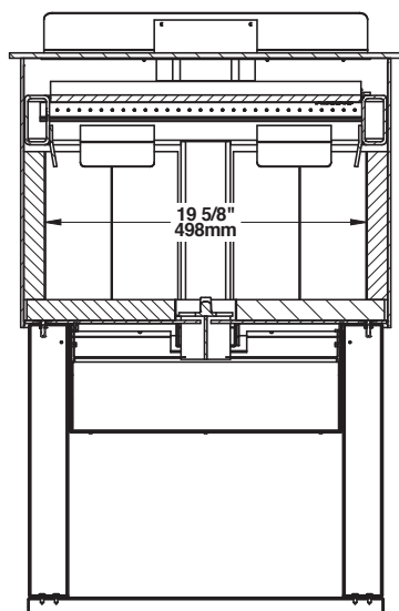
Combustion chamber - front view
